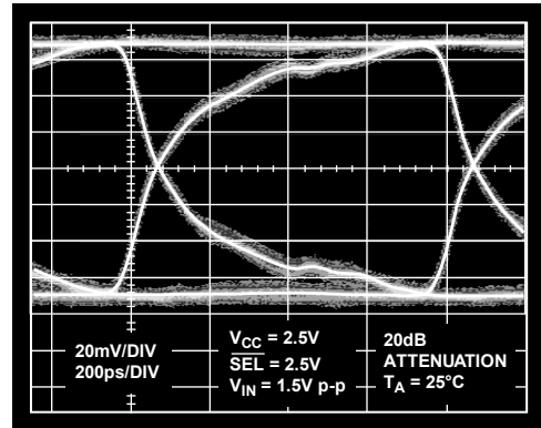
Figure 23. Eye Pattern; 1.244 Gbps, V_{CC} = 2.5\text{ V} , PRBS 31
