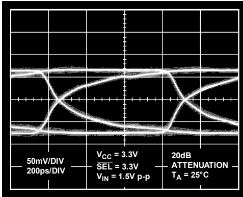
Figure 22. Eye Pattern; 1.5 Gbps, V_{CC} = 3.3\text{ V} , PRBS 31
