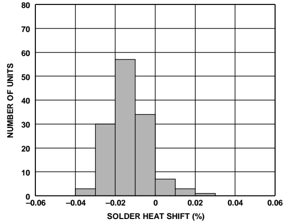
Figure 42. ADR4530 Solder Heat Resistance Shift (3 x Reflow)
