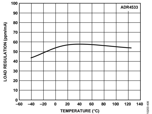
Figure 47. ADR4533 Load Regulation vs. Temperature (Sinking)
