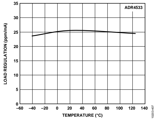
Figure 46. ADR4533 Load Regulation vs. Temperature (Sourcing)
