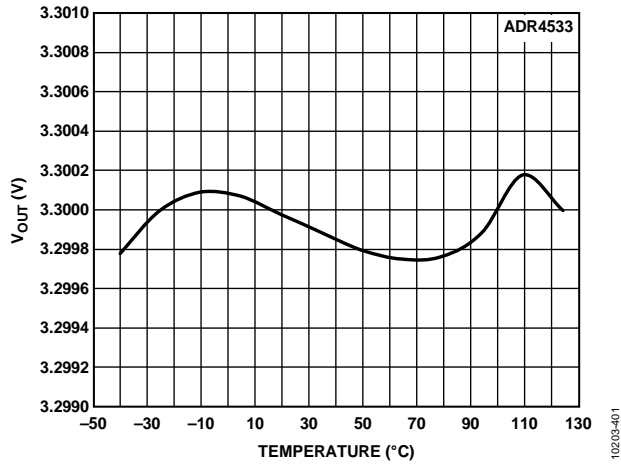
Figure 43. ADR4533 B Grade Output Voltage vs. Temperature
