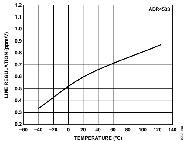
Figure 48. ADR4533 Line Regulation vs. Temperature
