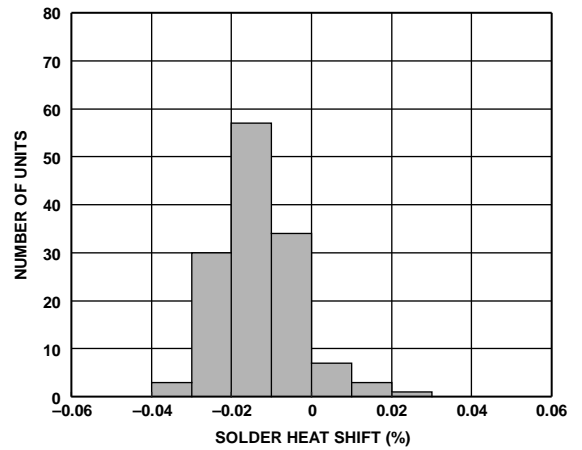
Figure 29. ADR4525 Solder Heat Resistance Shift (3 × Reflow)
