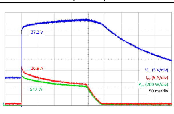
Figure 14. ISO 16750-2 test B response ( U_A + U_s^* = 13.5 + 30\text{ V} , U_s = 87\text{ V} , t_d = 400\text{ ms} , R_i = 0.5\text{ Ω} )
