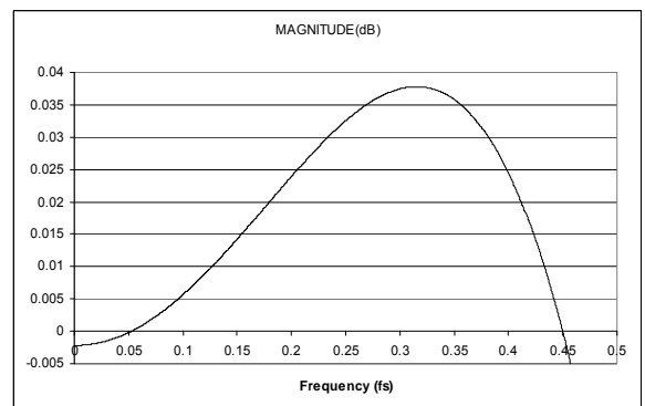
Figure 41 DAC Digital Filter Ripple (Normal Mode)
