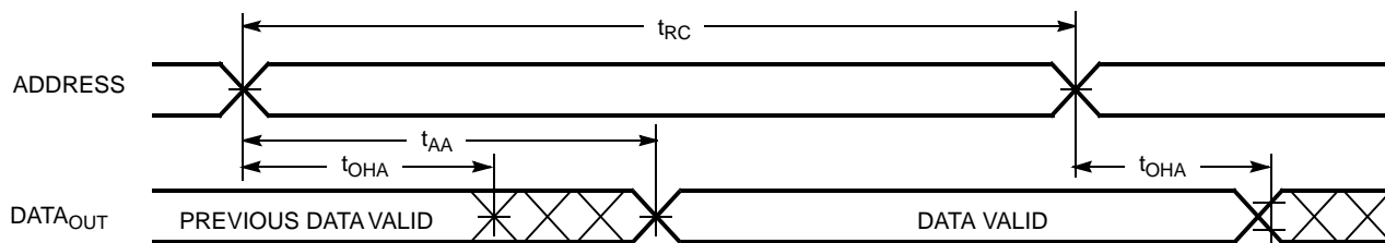
Figure 4. Read Cycle No.2 (Either Port \overline{CE}/\overline{OE} Access) [16, 19, 20]
