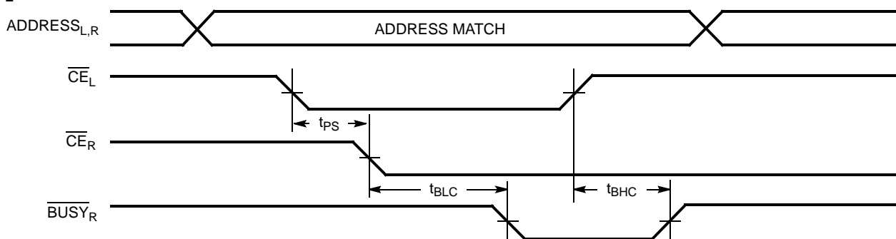
Figure 12. Busy Timing Diagram No. 1 ( \overline{\text{CE}} Arbitration) [35]
