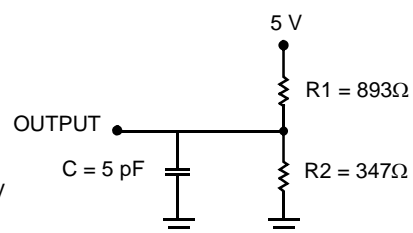
(c) Three-State Delay (Load 2) (Used for t_{LZ} , t_{HZ} , t_{HZWE} , & t_{LZWE} including scope and jig)
