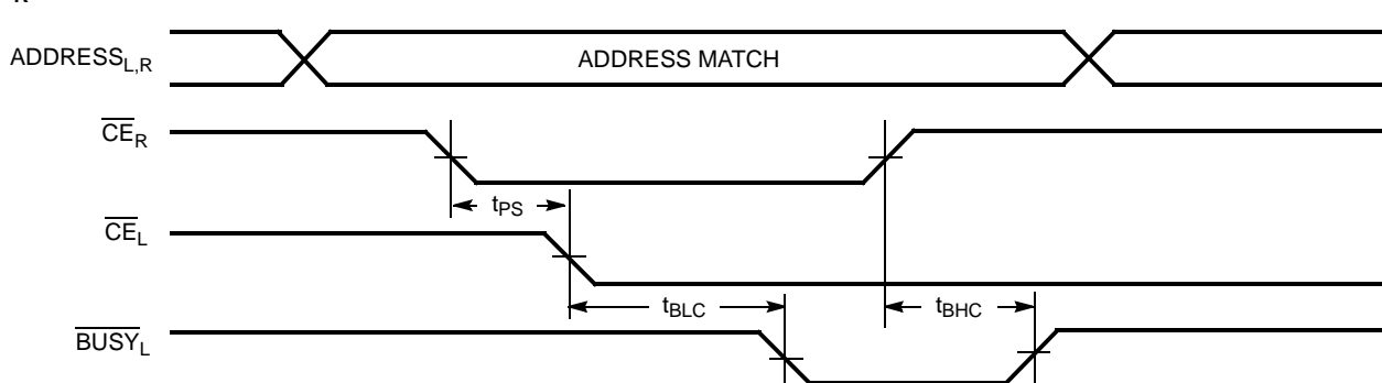
Figure 13. Busy Timing Diagram No. 2 (Address Arbitration) [35]
