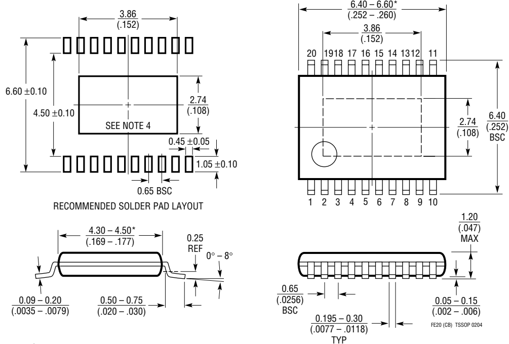
FE Package 20-Lead Plastic TSSOP (4.4mm) (Reference LTC DWG # 05-08-1663) Exposed Pad Variation CB
