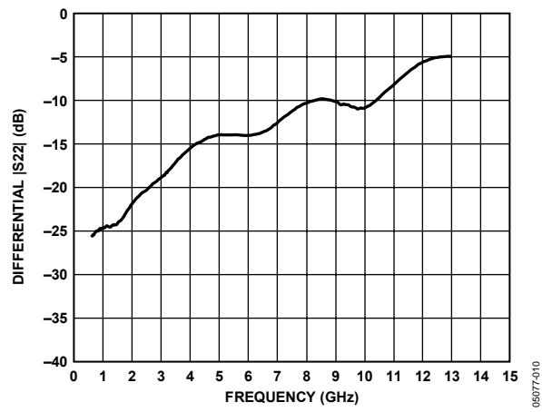
Figure 11. Differential |S22|
