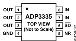
Figure 3. 8-Lead MSOP
