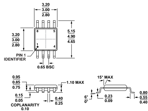
Figure 27. 8-Lead Mini Small Outline Package [MSOP] (RM-8)
