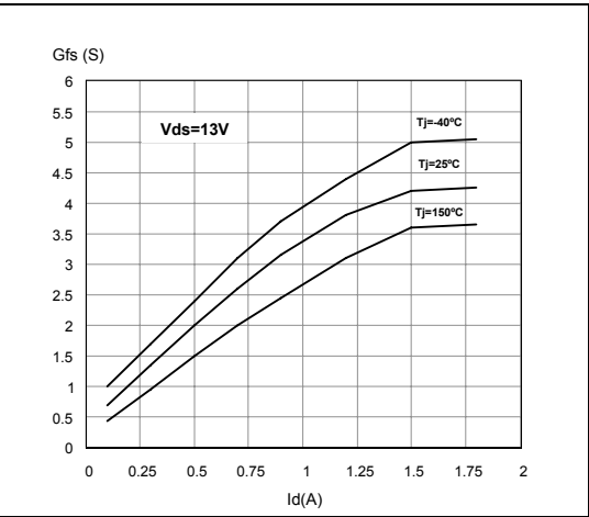
Figure 14. Transconductance
