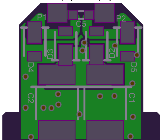
Figure 37 Top Layer
