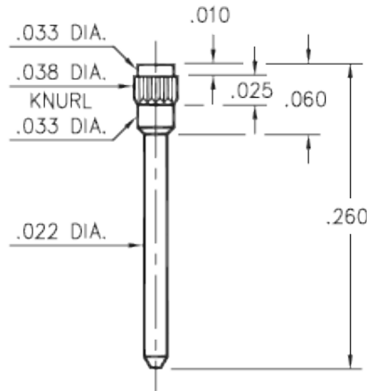
7827-0-00-XX-00-00-03-0 Press-fit in .035 mounting hole
