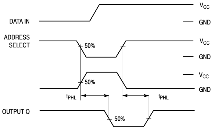
Figure 7. Switching Waveform
