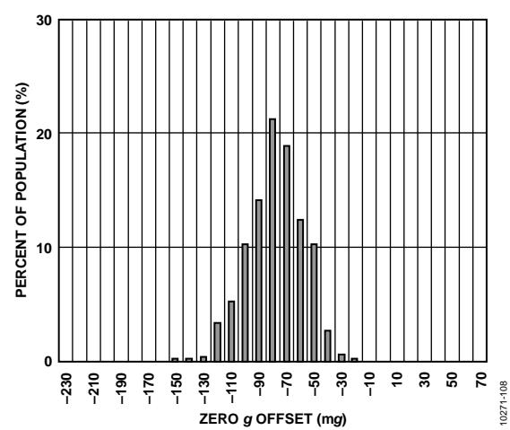
Figure 9. Z-Axis Zero g Offset at 25°C, V_S = 3.0 V
