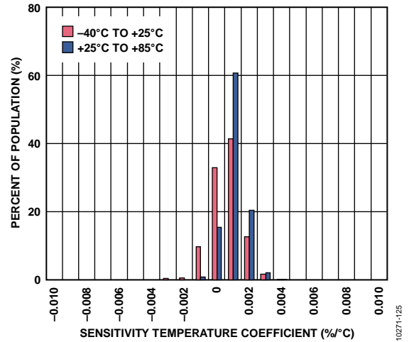
Figure 26. Y-Axis Sensitivity Temperature Coefficient, V_s = 2.5\text{ V}
