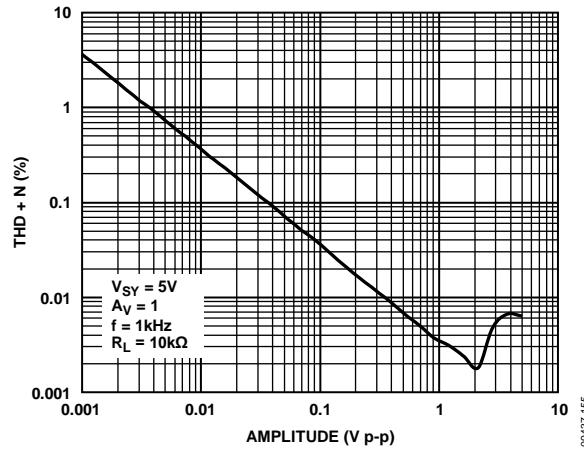
Figure 59. THD + N vs. Amplitude
