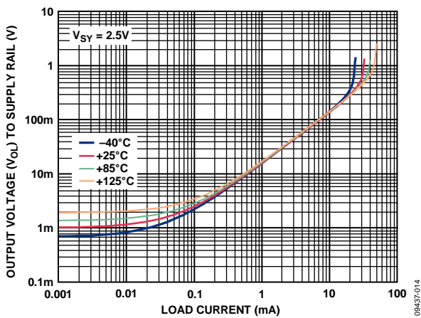
Figure 15. Output Voltage ( V_{O1} ) to Supply Rail vs. Load Current
