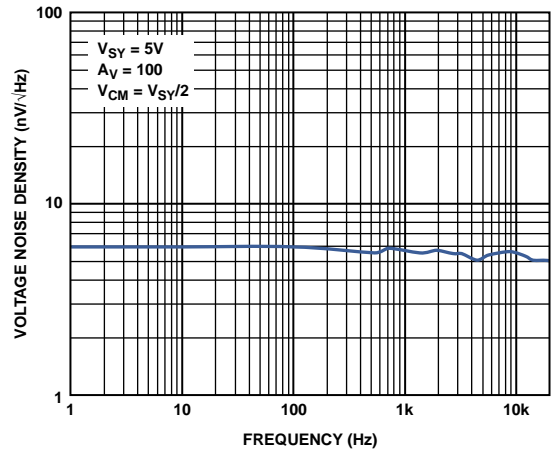
Figure 53. Voltage Noise Density vs. Frequency
