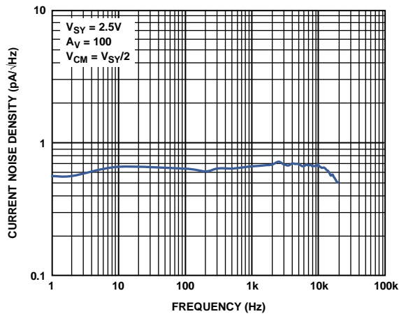
Figure 51. Current Noise Density vs. Frequency
