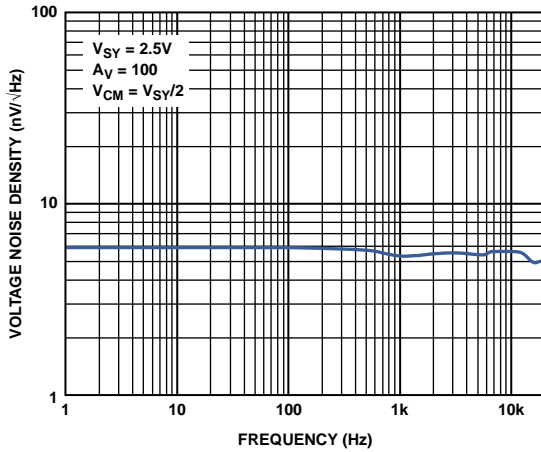
Figure 50. Voltage Noise Density vs. Frequency
