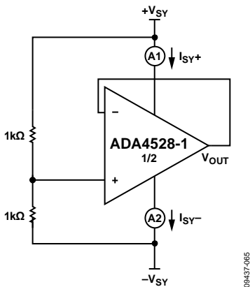
Figure 65. Voltage Follower
