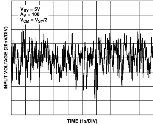
Figure 58. 0.1 Hz to 10 Hz Noise
