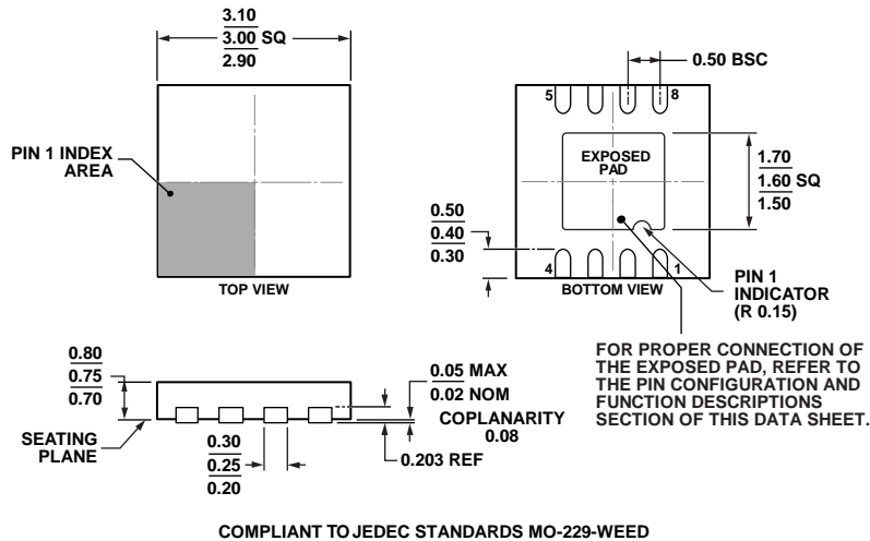
COMPLIANT TO JEDEC STANDARDS MO-229-WEED Figure 72. 8-Lead Lead Frame Chip Scale Package [LF CSP_WD] 3 mm x 3 mm Body, Very Very Thin, Dual Lead (CP-8-12) Dimensions shown in millimeters
