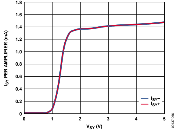
Figure 66. Supply Current vs. Supply Voltage (Voltage Follower)
