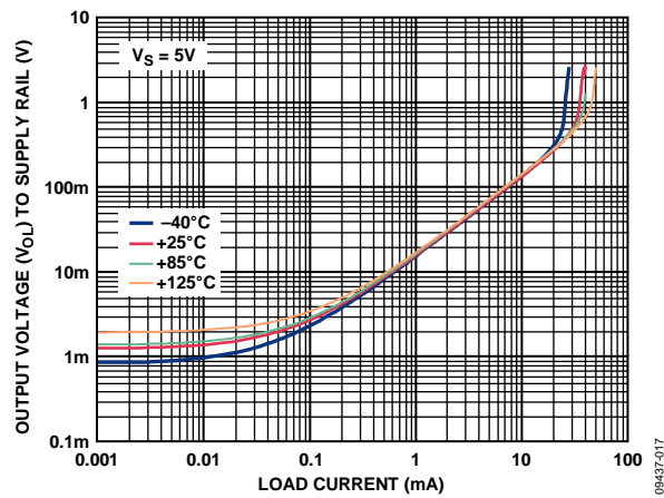
Figure 18. Output Voltage ( V_{O1} ) to Supply Rail vs. Load Current
