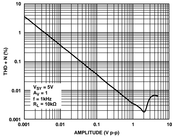
Figure 59. THD + N vs. Amplitude
