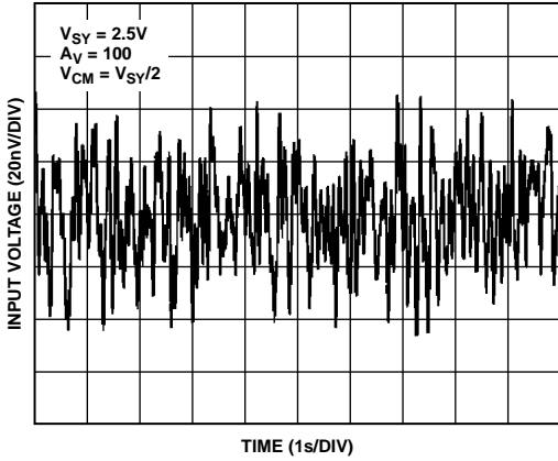
Figure 55. 0.1 Hz to 10 Hz Noise
