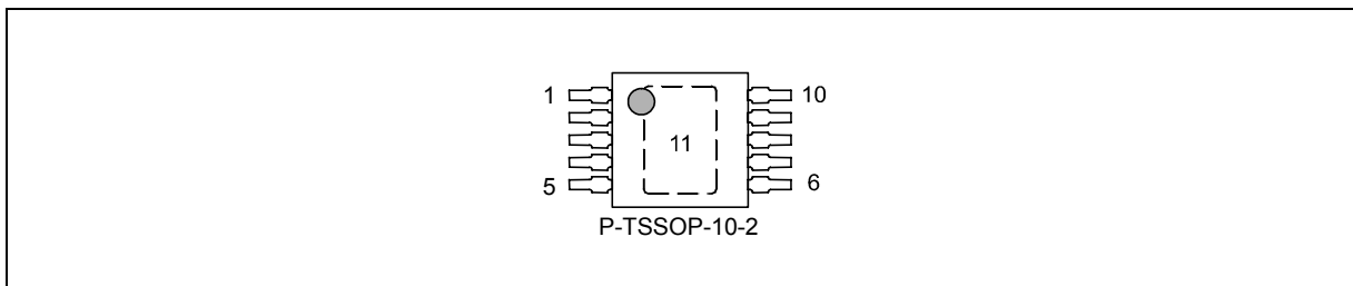
Figure 3 CGB240B Outline
