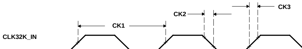
Figure 5–4. 32-kHz Input Clock
