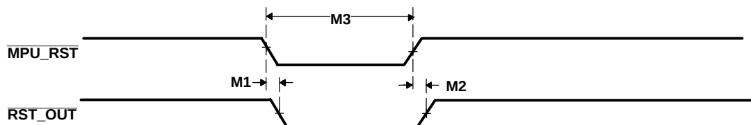
Figure 5–8. MPU Core Reset Timings
