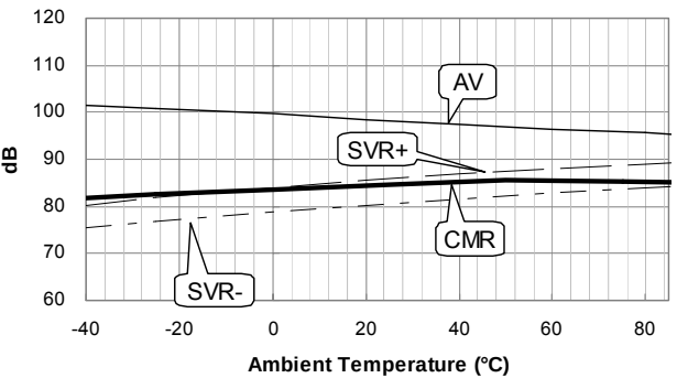
Amp.Gain vs. Ambient Temperature ( Bch )
