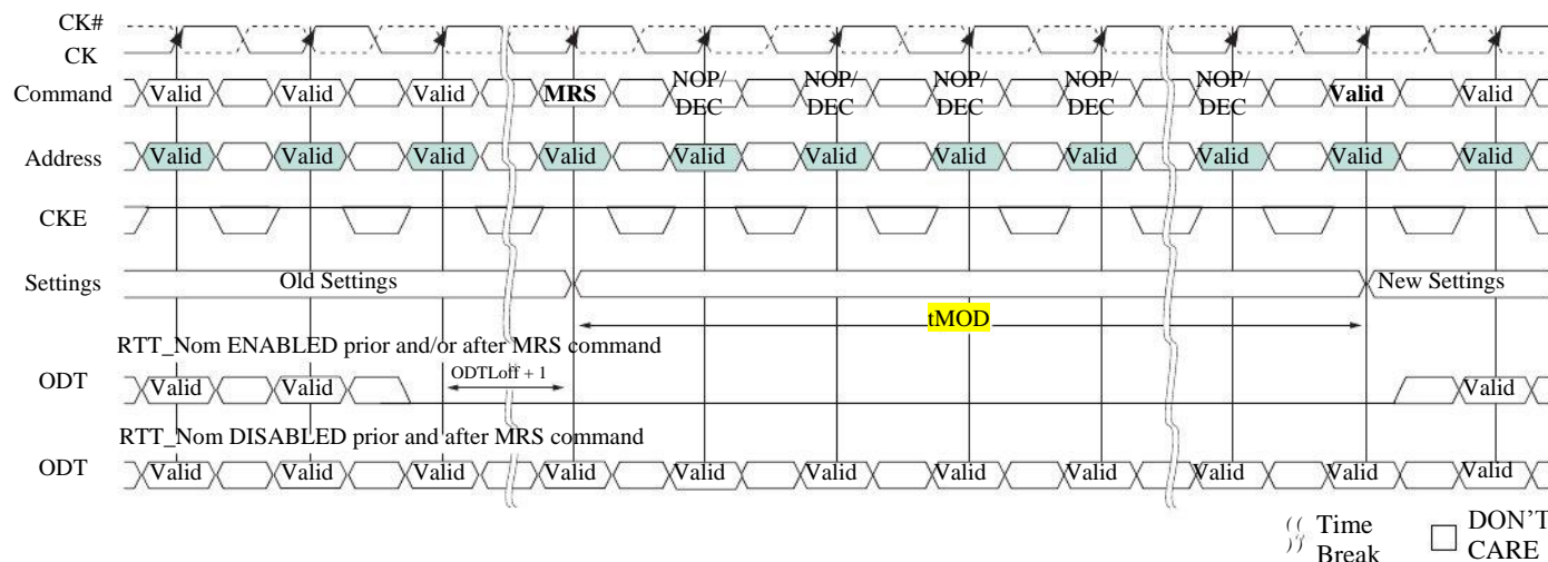
The mode register contents can be changed using the same command and timing requirements during normal operation as long as the DRAM is in idle state, i.e., all banks are in the precharged state with tRP satisfied, all data bursts are completed and CKE is high prior to writing into the mode register. If the RTT_NOM Feature is enabled in the Mode Register prior and/or after an MRS Command, the ODT Signal must continuously be registered LOW ensuring RTT is in an off State prior to the MRS command. The ODT Signal maybe registered high after tMOD has expired. If the RTT_NOM Feature is disabled in the Mode Register prior and after an MRS command, the ODT Signal can be registered either LOW or HIGH before, during and after the MRS command. The mode registers are divided into various fields depending on the functionality and/or modes.
