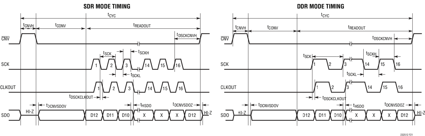
Figure 21. LTC2325-12 Timing Diagram
