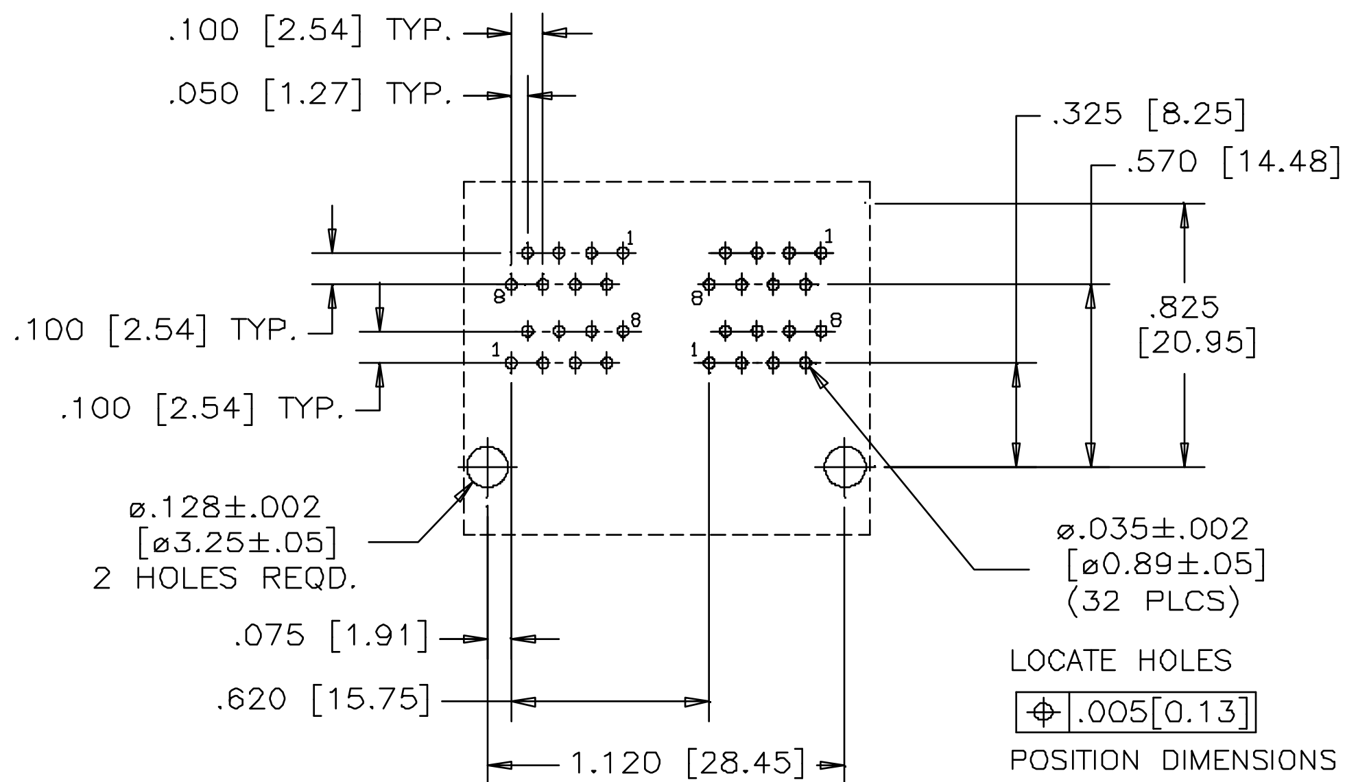
RECOMMENDED P.C.B. LAYOUT (COMPONENT SIDE OF BOARD)
