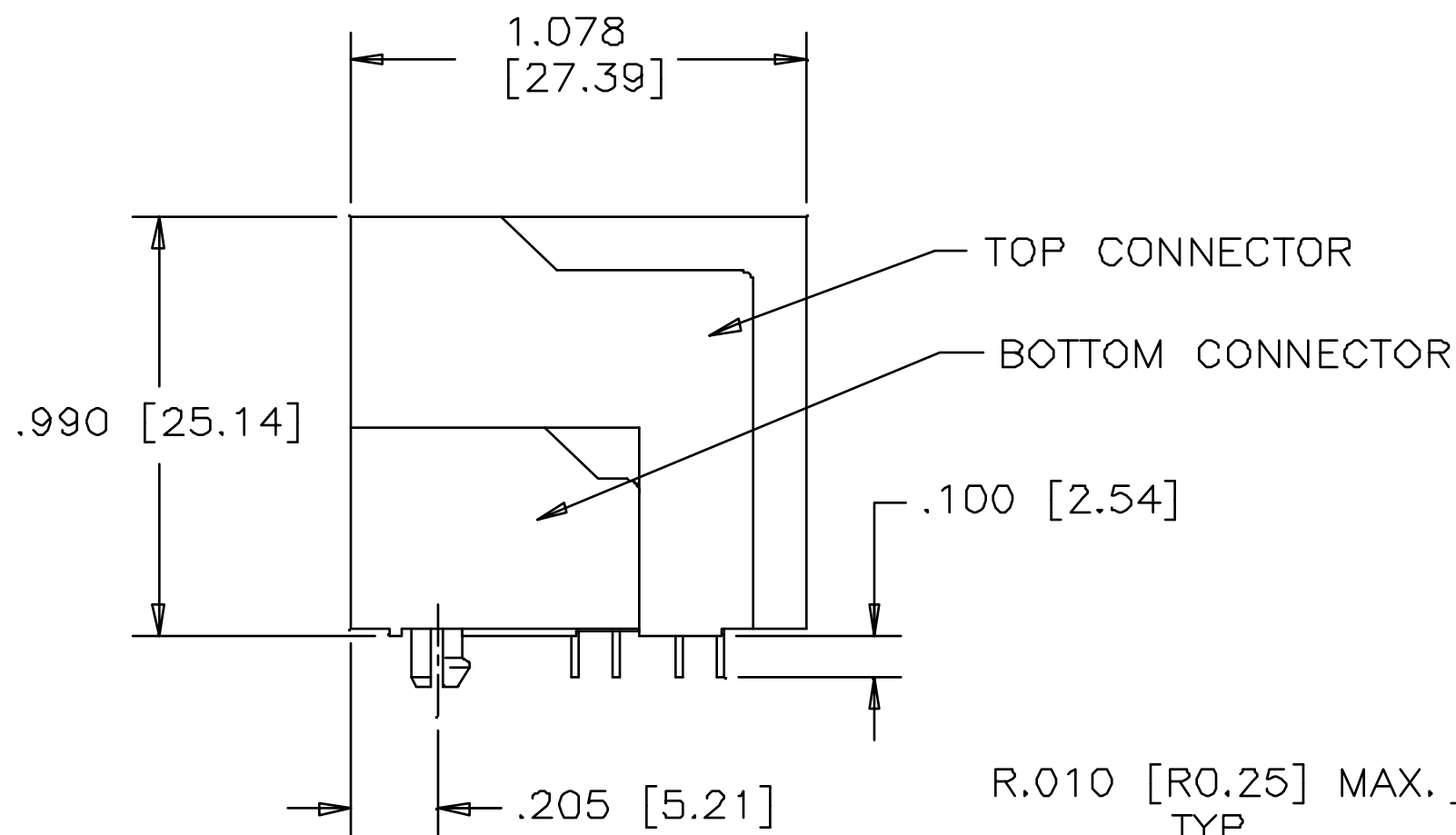
SIDE VIEW
