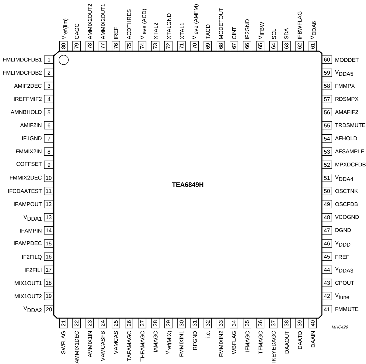
Fig.2 Pin configuration.
