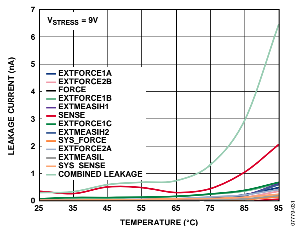
Figure 19. Leakage Current vs. Temperature (Force and Combined Leakage), V_{\text{STRESS}} = 9V
