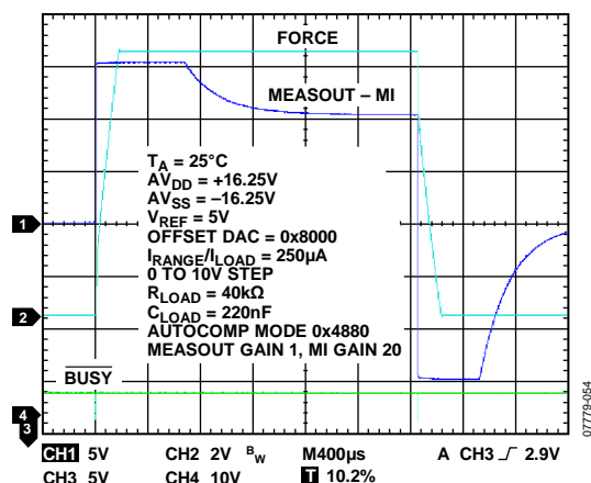
Figure 40. Transient Response FVMI Mode, ±250 \mu A Range, Autocompensation Mode
