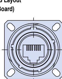
Receptacle Front View
