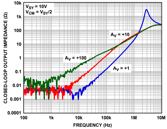
Figure 59. Closed-Loop Output Impedance vs. Frequency
