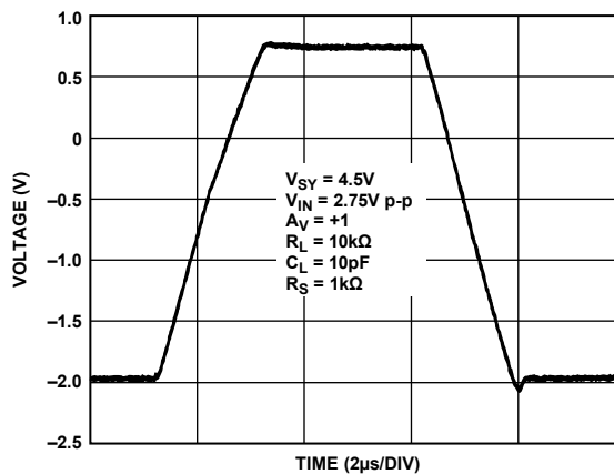
Figure 64. Large Signal Transient Response, V_{SY} = 4.5\text{ V}
