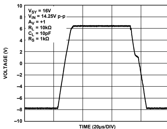
Figure 66. Large Signal Transient Response, V_{SY} = 16\text{ V}
