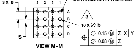
VIEW M-M
