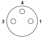
Pin assignment of M8 female connector, 3-pos., view of pin side
