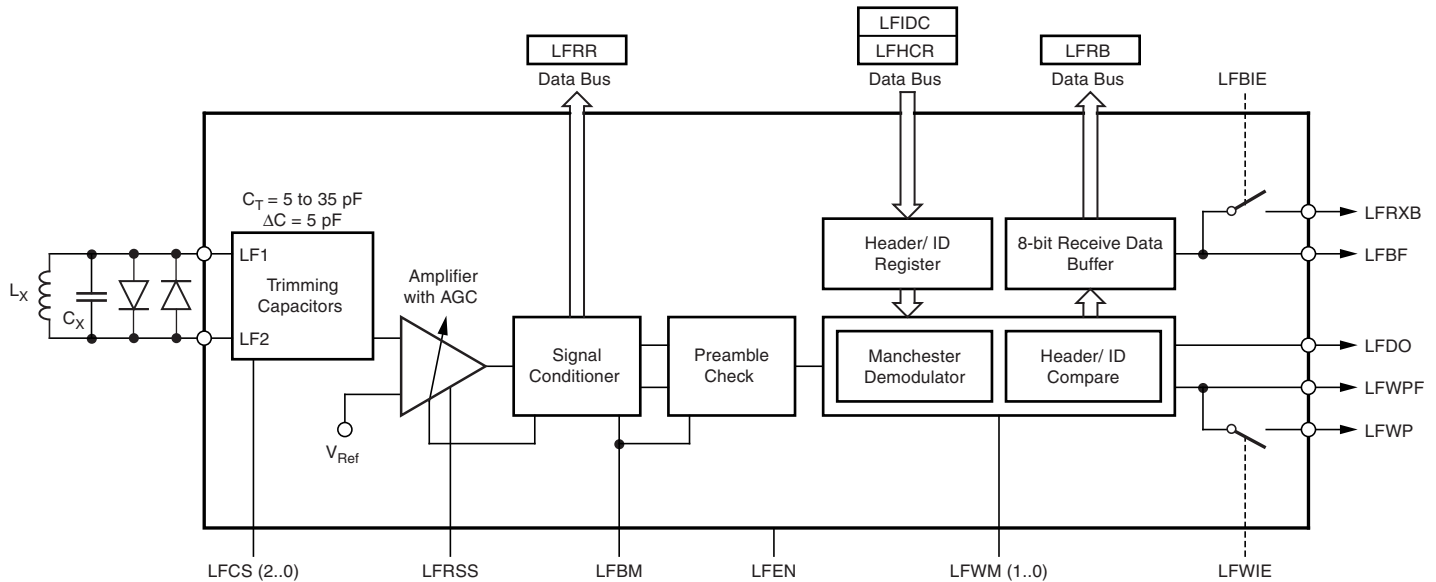
Figure 3-65. LF Receiver Block
