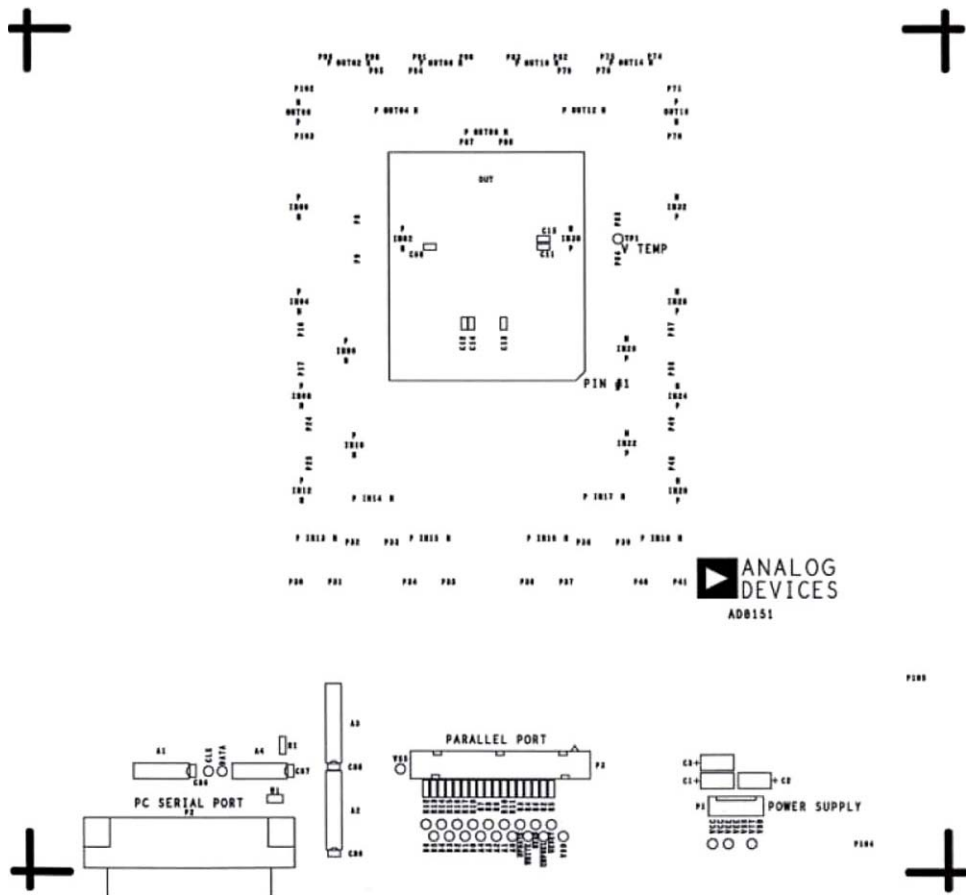
Figure 45. Silkscreen Top
