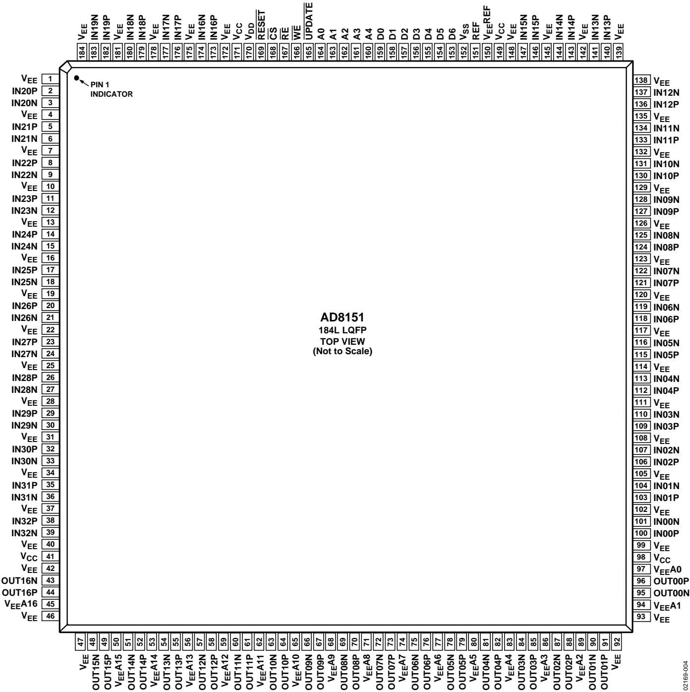
Figure 4. Pin Configuration
