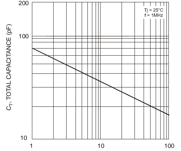
V R , REVERSE VOLTAGE (V) Fig. 4 Typical Total Capacitance
