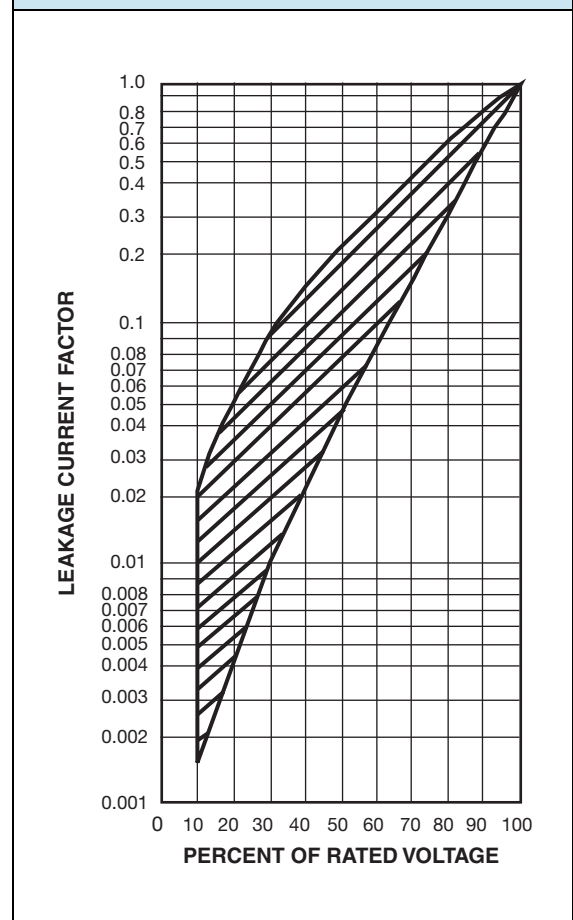
LEAKAGE AS A FUNCTION OF VOLTAGE AND TEMPERATURE
