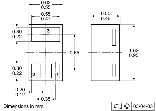
Fig 8. Package outline BAV70M (SOT883/SC-101)
