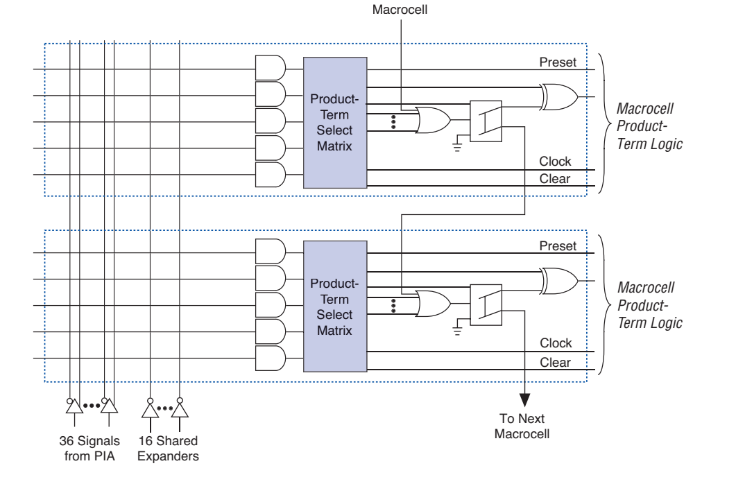
Unused product terms in a macrocell can be allocated to a neighboring macrocell.
