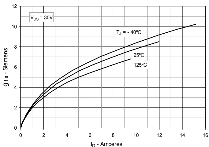
Fig. 10. Transconductance
