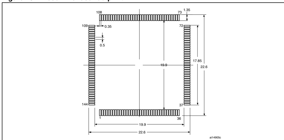
Figure 78. Recommended footprint
