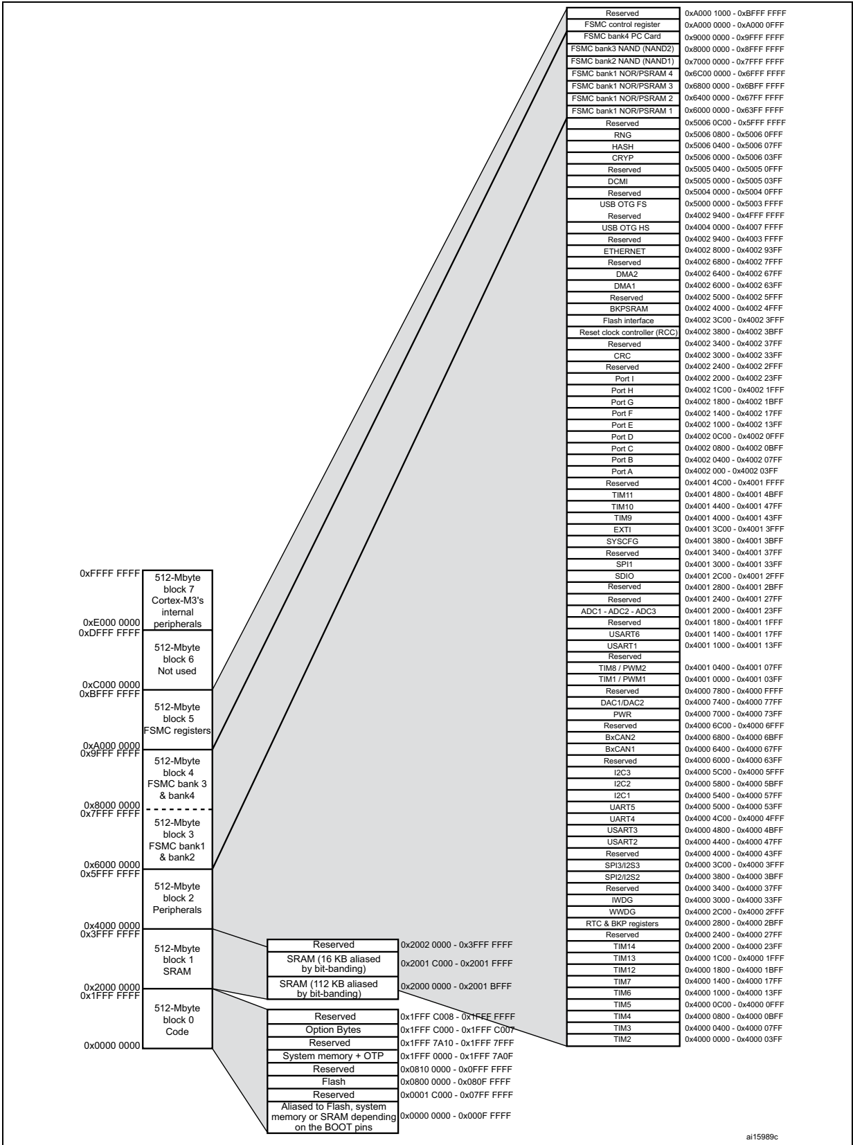
Figure 13. Memory map
