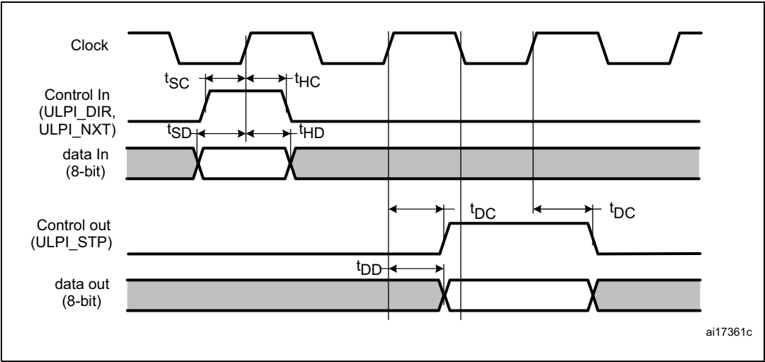
Figure 44. ULPI timing diagram
