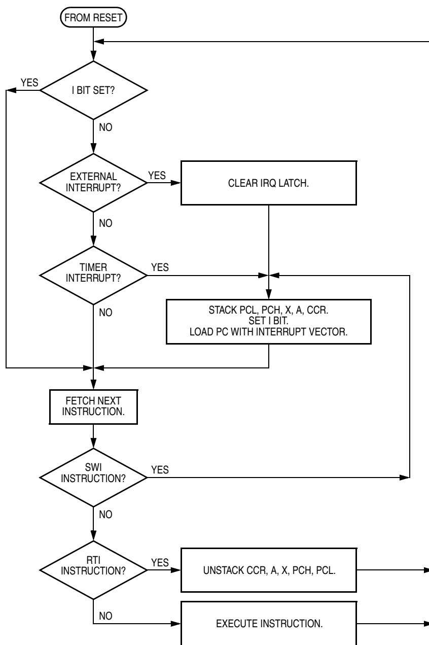
Figure 5-3. Interrupt Flowchart
