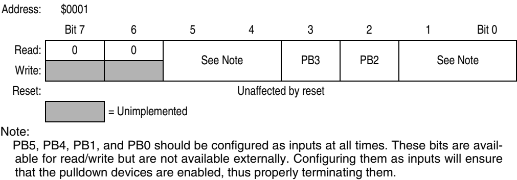
Figure 7-6. Port B Data Register (PORTB)
