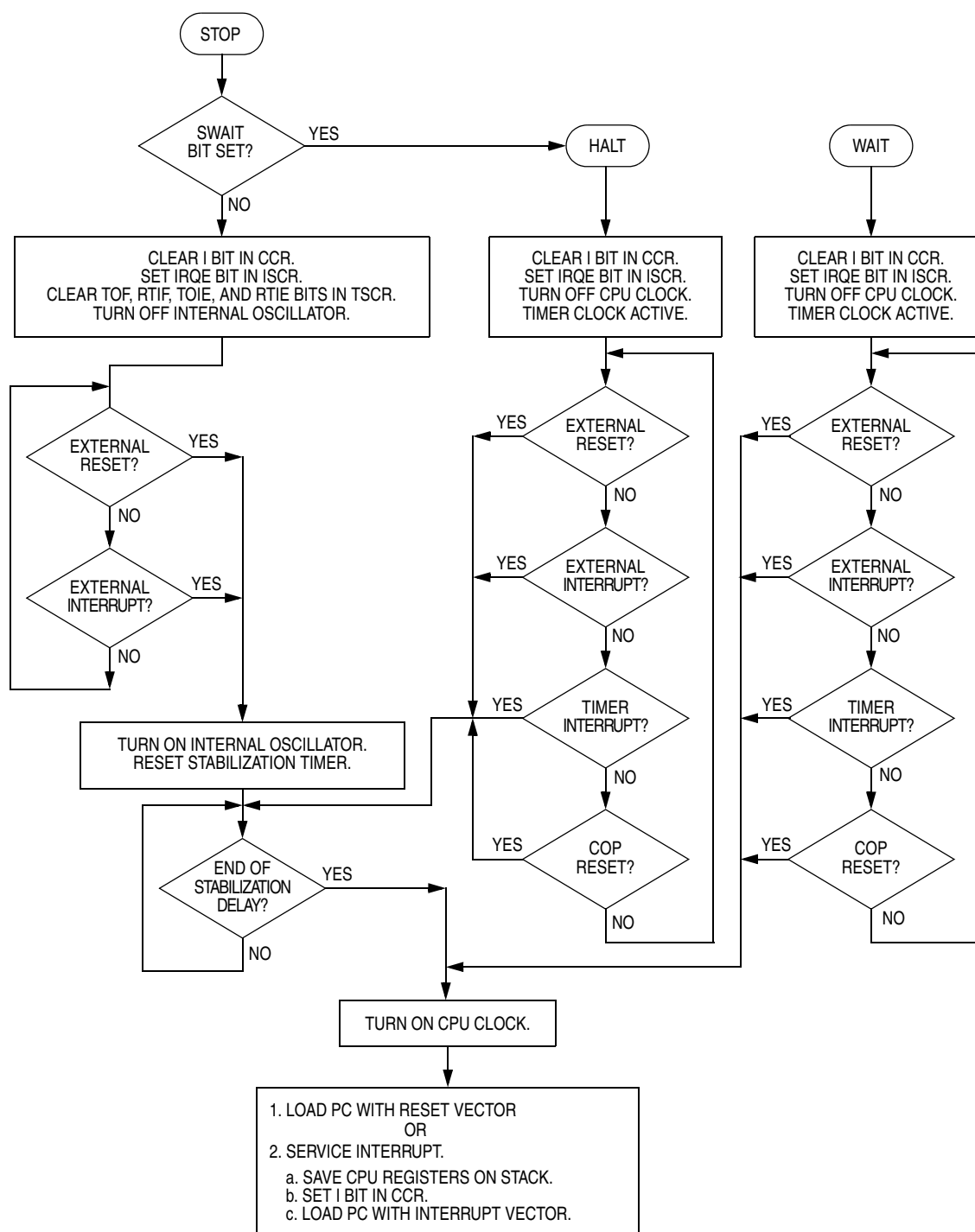
Figure 6-2. STOP/HALT/WAIT Flowchart
