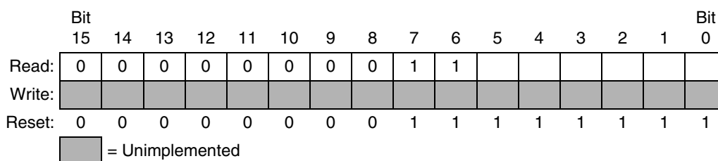
Figure 4-4. Stack Pointer (SP)
