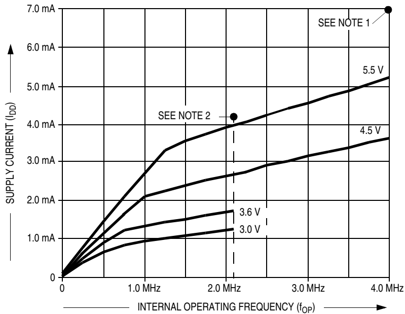
Figure 10-5. Typical Operating I_{DD} (25°C)
