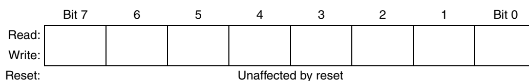
Figure 4-2. Accumulator (A)
