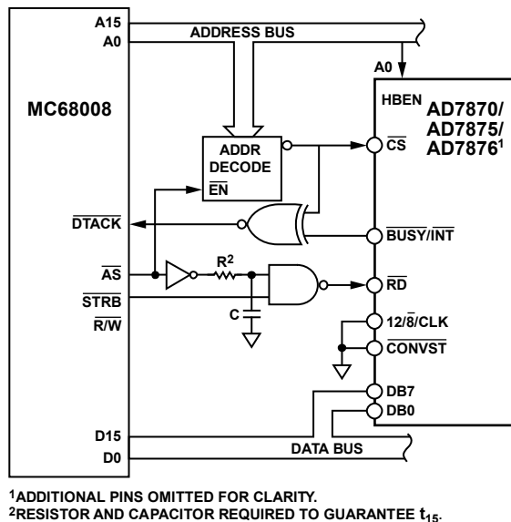
Figure 25. MC68008 Byte Interface
