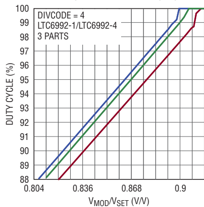
Linearity Near 100% Duty Cycle
