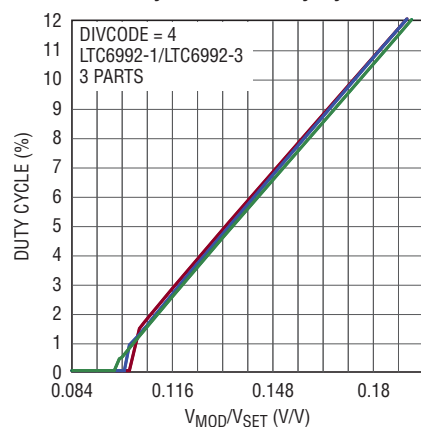
Linearity Near 0% Duty Cycle
