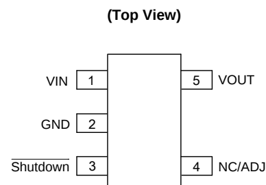
(SOT-23-5)
