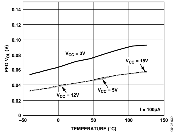
Figure 36. PFO Output Low Voltage vs. Temperature, I = 100 \mu A
