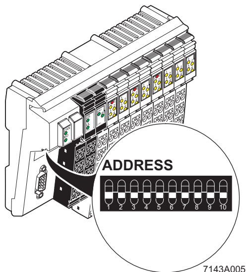
Figure 4 DIP switches of the module
