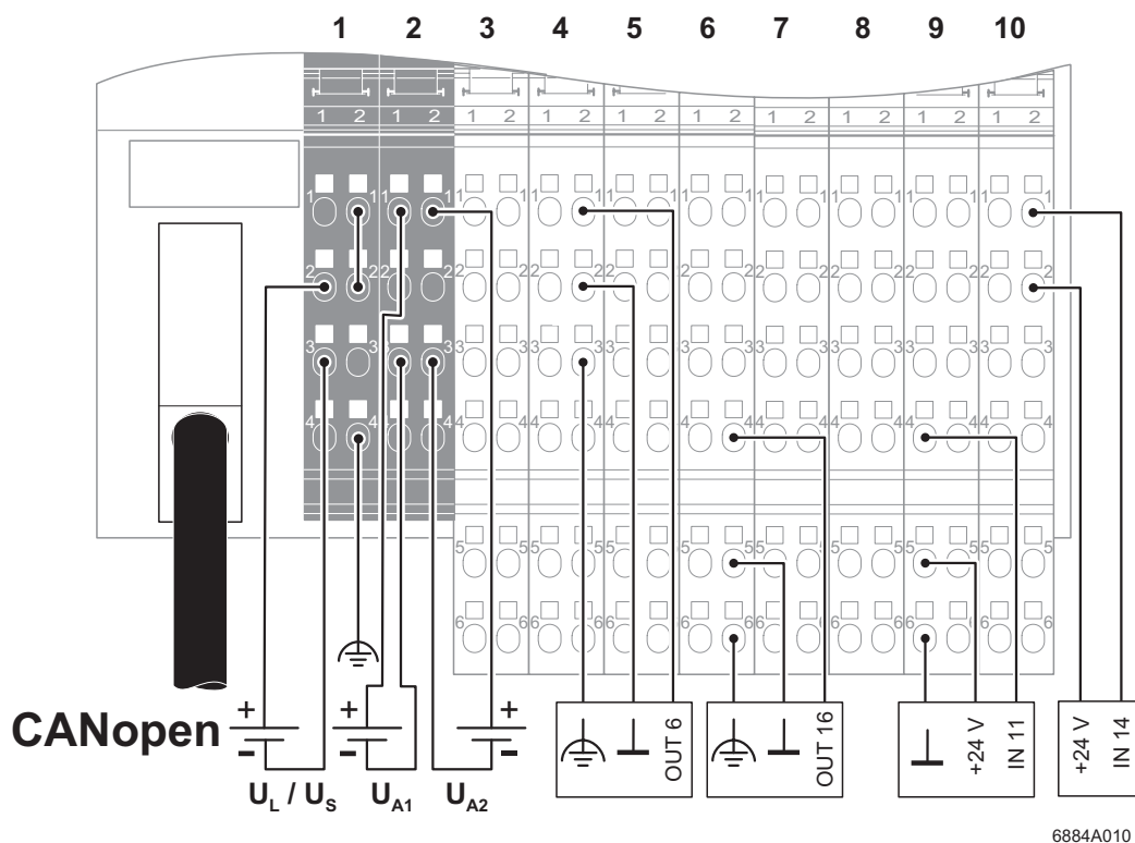
Figure 7 Connection example
