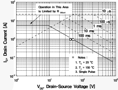
Figure 9-2. Maximum Safe Operating Area for FQPF6N80C
