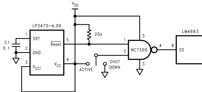
FIGURE 2. At power-up, the LP3470 forces the LM4663 into shutdown, which prevents abnormal quiescent current flow through the amplifier. Once V CC rises above 4V and after a 200ms delay set by C1, normal amplifier operation is restored.
