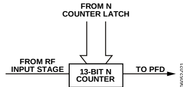
Figure 12. N Counter
