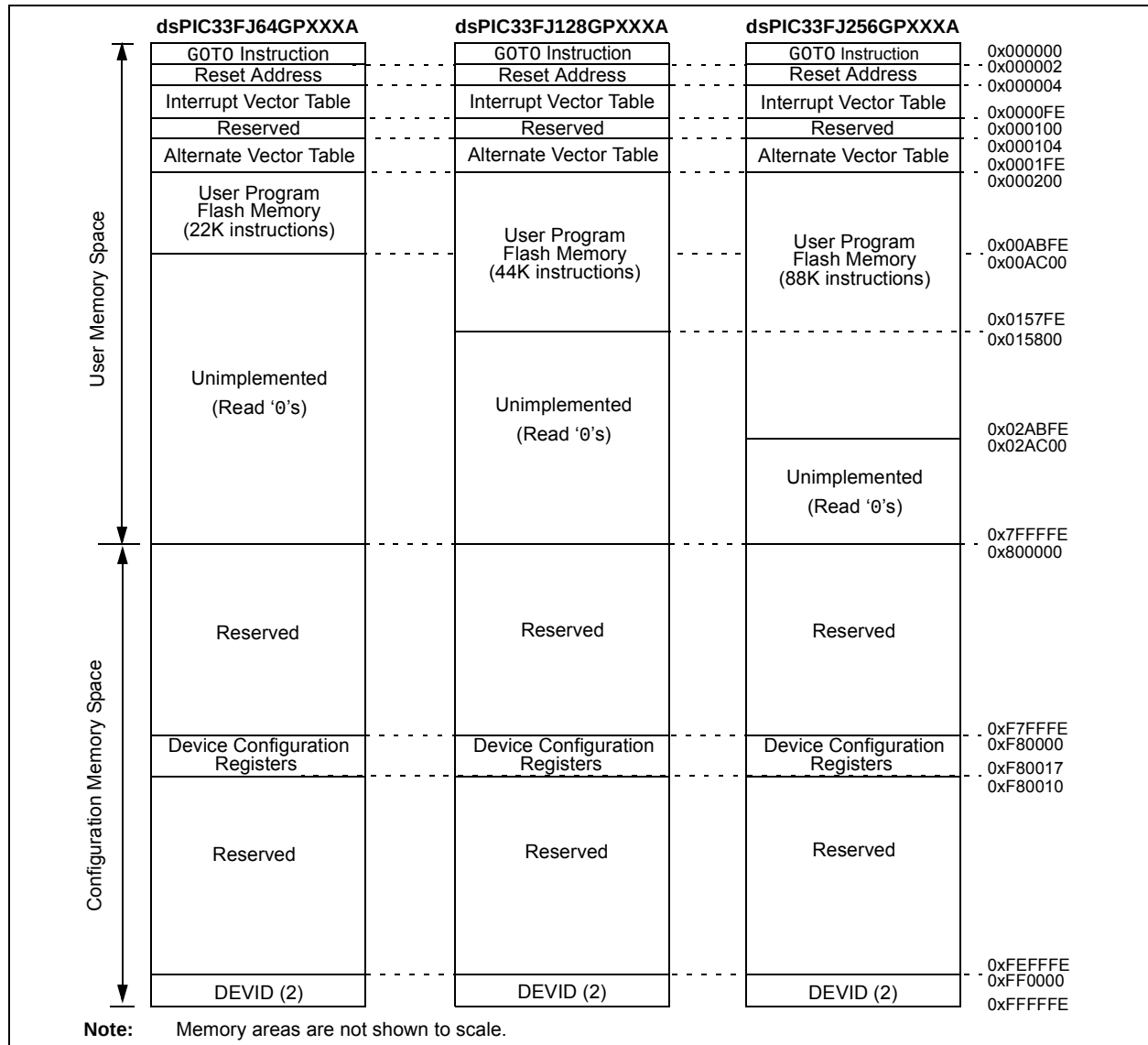
FIGURE 4-1: PROGRAM MEMORY FOR dsPIC33FJXXGXP06A/X08A/X10A DEVICES
