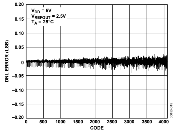
Figure 15. AD5624R-5 DNL, Internal Reference
