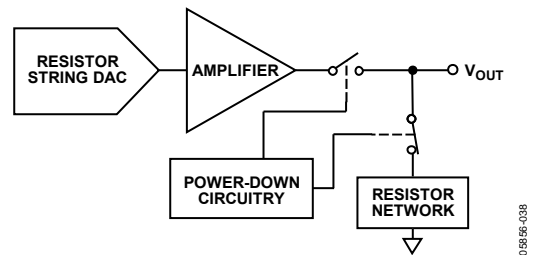
Figure 56. Output Stage During Power-Down
