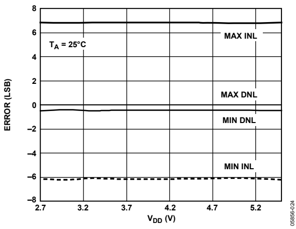
Figure 24. INL Error and DNL Error vs. Supply
